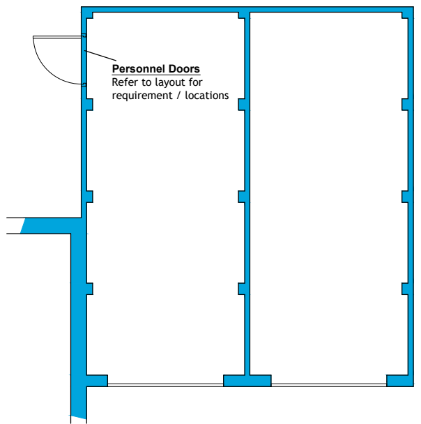
Floor Plan DG1 (Single Garages)
